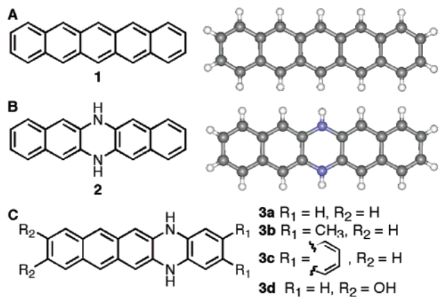
Figure 1. (a) Molecular structure and crystal structure of pentacene 7 (1); (b) molecular structure and crystal structure of 2, 6,13-dihydrodiazapentacene; and (c) derivatives of 5,14-dihydrodiazapentacene (3a–d).
